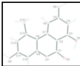
Fig. 1. : ORTEP representation of the title compound with atomic labeling shown with 30% probability displacement ellipsoids.
